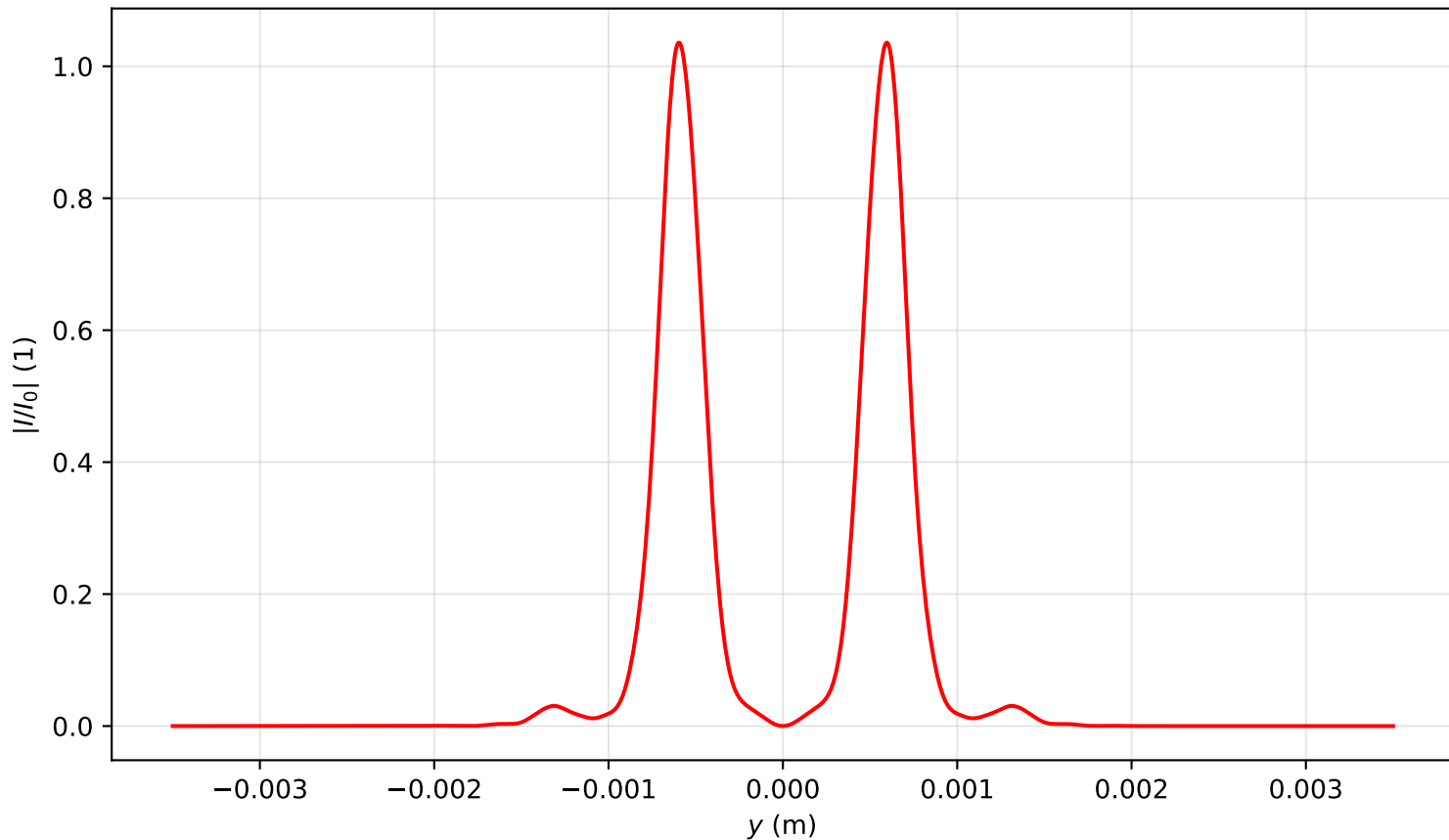
Intensity profile I(x=0, y, z=0.955)/I_0 , P_{in}=7.0P_{cr} , artificial time
